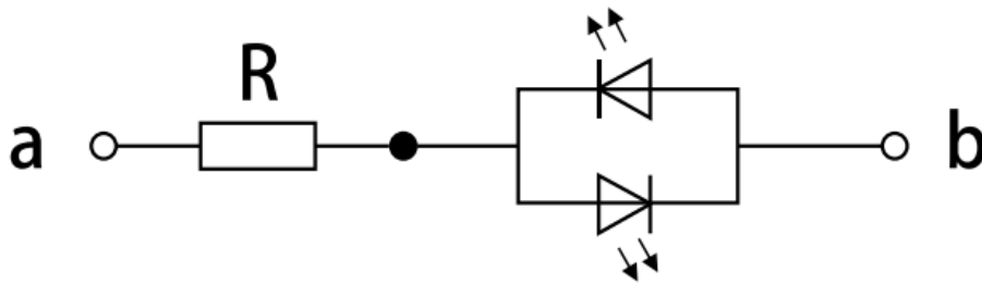
Lamp Circuit diagram
