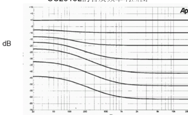
SC2313L响度于音量衰减频率响应 (C10=C11=100nF)
